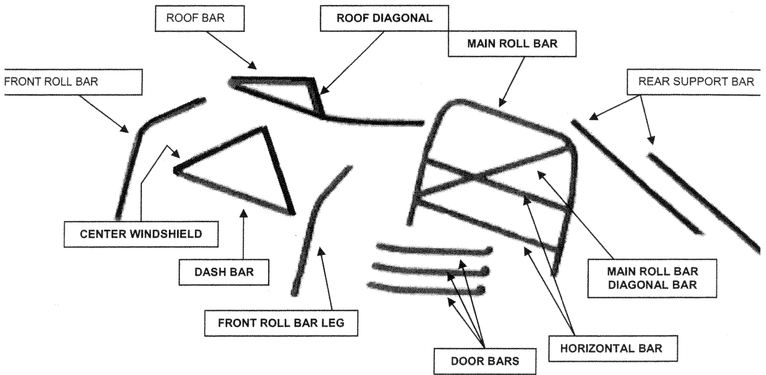
ROLL CAGE CONSTRUCTION DIAGRAM
